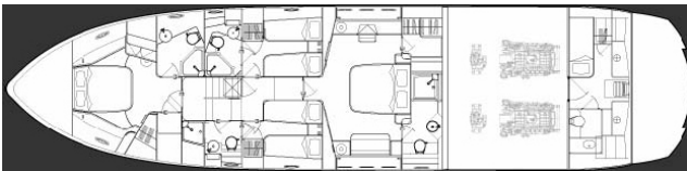
Layout accommodation
